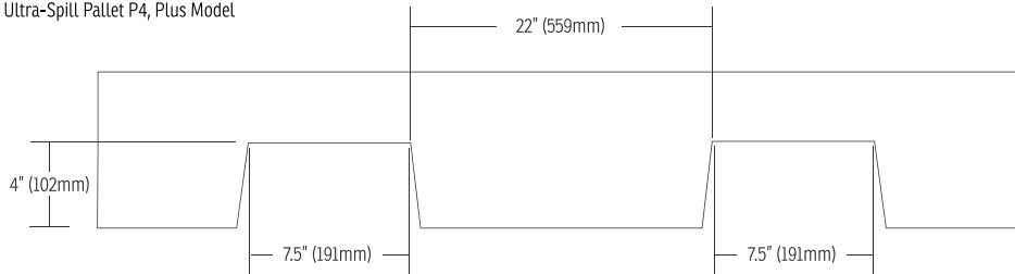
Forklift Pocket Dimensions for: Ultra-Spill Pallet P4, Plus Model
