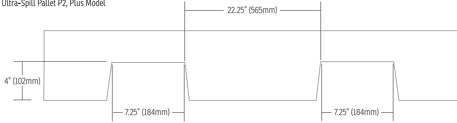
Forklift Pocket Dimensions for: Ultra-Spill Pallet P2, Plus Model
