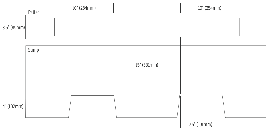
Forklift Pocket Dimensions for: Ultra-Spill King
