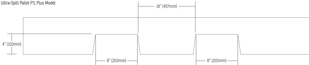
Forklift Pocket Dimensions for: Ultra-Spill Pallet P3, Plus Model
