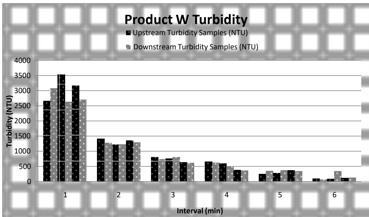
Figure 42: Sample water turbidity for 3 rainfall events on Product W over time
