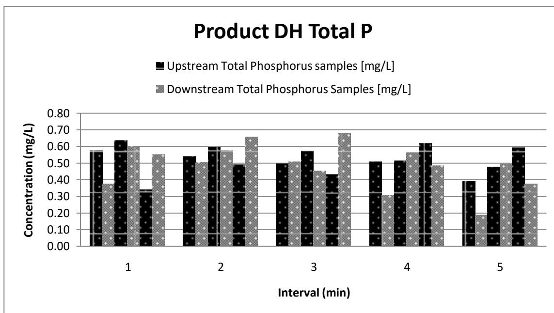
Figure 113: Sample water TP for 3 rainfall events on Product DH over time
