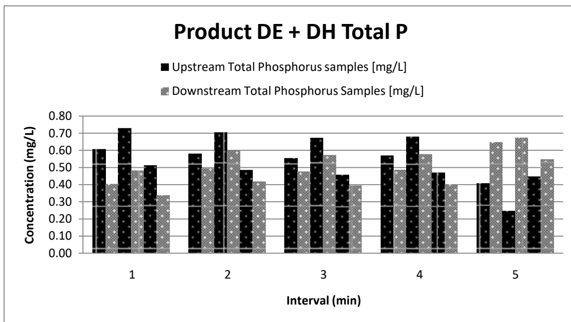
Figure 118: Sample water TP for 3 rainfall events on Product DE + DH over time
