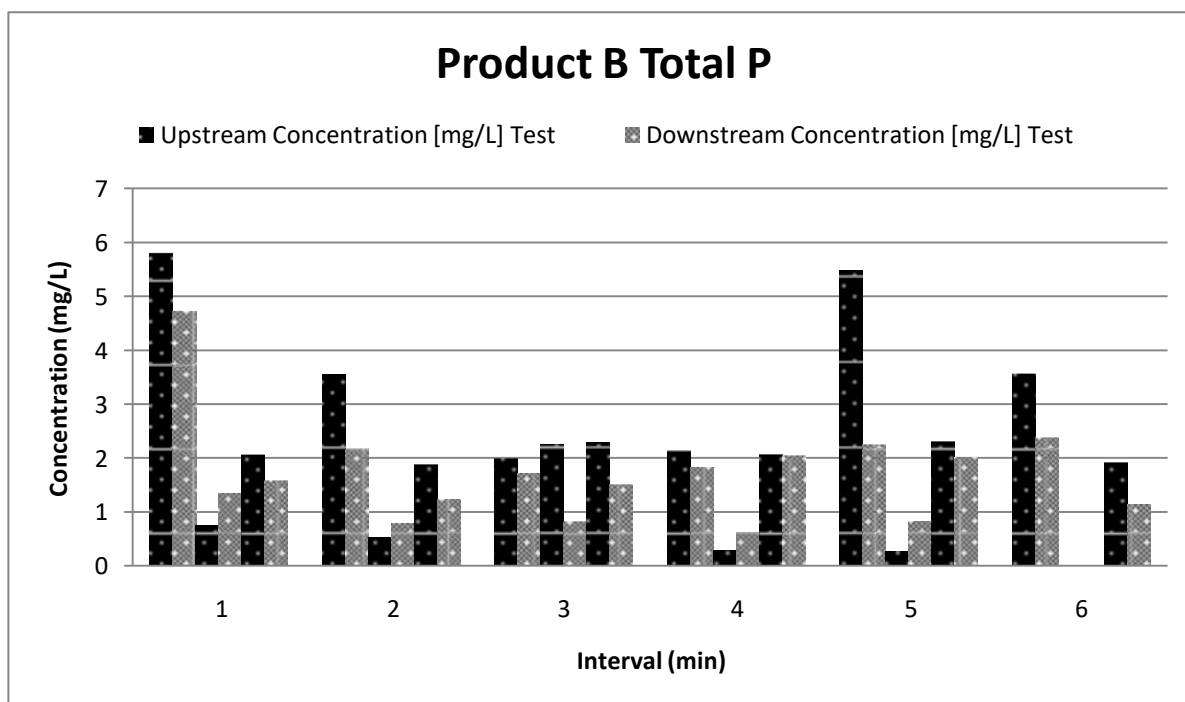
Figure 64: Sample water TP concentration for 3 rainfall events on Product B over time
