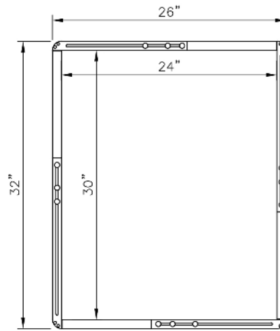
ADJUSTABLE FRAME MAXIMUM INLET SIZE (24"X30")
