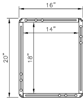
ADJUSTABLE FRAME MINIMUM INLET SIZE (14"X18")
