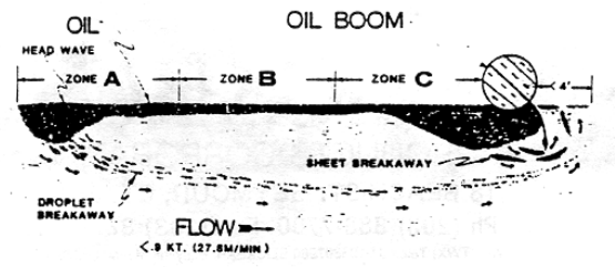
FIGURE 1-11 CONFIGURATION OF OIL AGAINST BOOM
