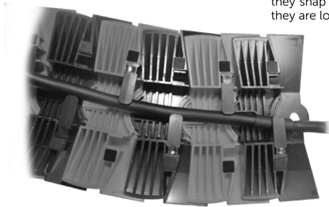
Figure 3: Medium and Large sizes use retainers to secure cables in place
