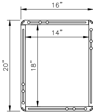
ADJUSTABLE FRAME MINIMUM INLET SIZE (14"X18")
