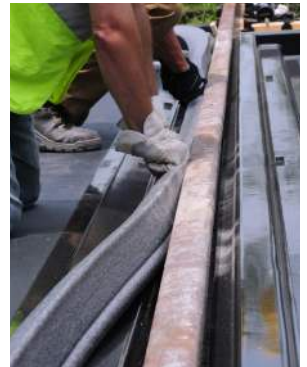
Optional rail side gaskets prevent leaking between rails and Track Pans.
